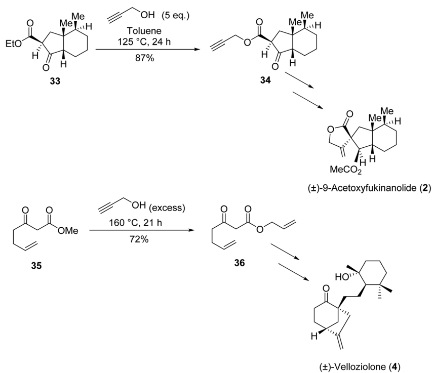
Scheme 9 Synthesis of (±)-9-acetoxifykunanolide and (±)-velloziolone.
