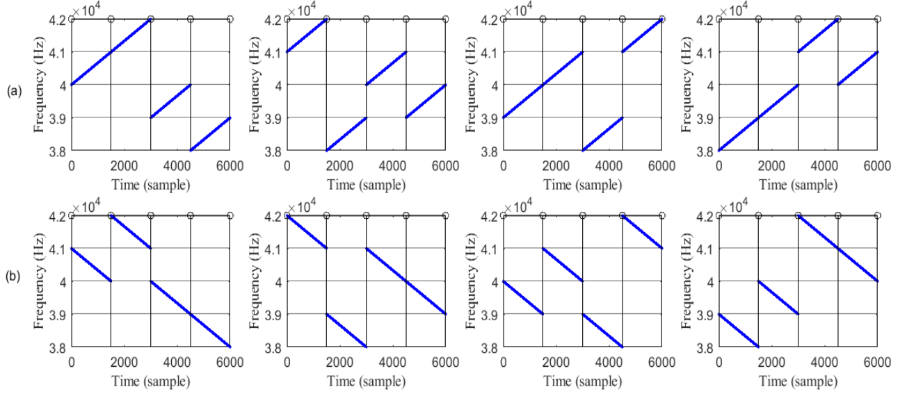
Fig. 3. (a) Four signals in set-1 after optimization and (b) the corresponding signals in the set-2
