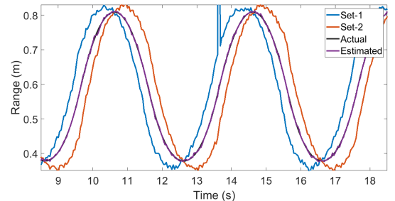
Fig. 9. The range estimated from the simulation experiment using signals from set-1, set-2 and Doppler-velocity correction method and the actual range at a simulated Doppler-velocity of 1m/s.
