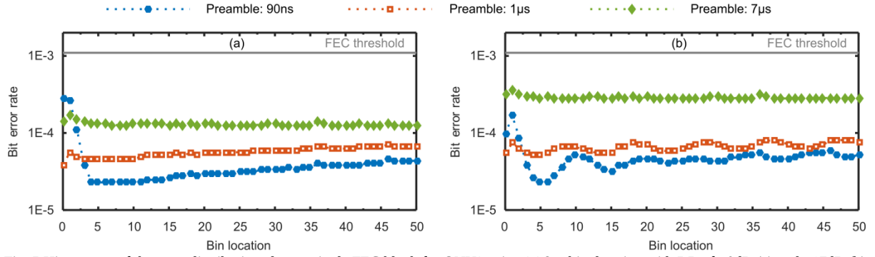
Fig. 5 Histograms of the error distribution along a single FEC block for ONU2 using 24.8ns bin duration with DR of \sim 0 dB (a) and \sim 17 dB (b).
