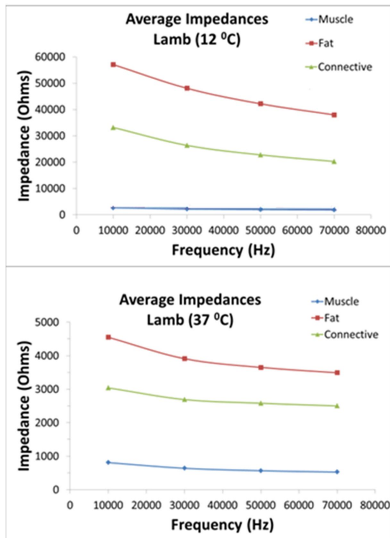
Figure 5.8: impedance values at different frequencies measured on lamb meat samples at 12°C and 37°C
