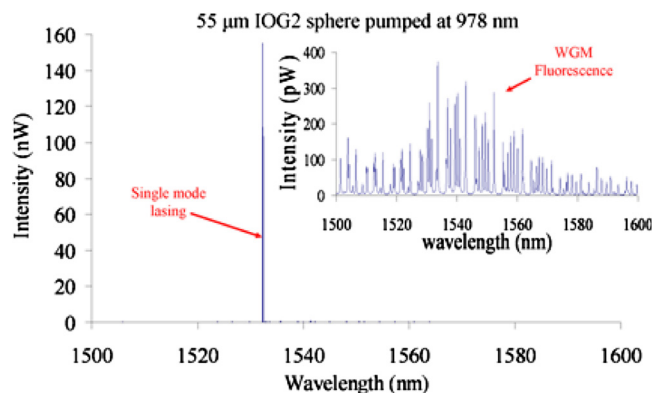
FIG. 4. (Color online) Single mode lasing at 1532\ \text{nm} from a 55\ \mu\text{m} IOG-2 microsphere pumped at 978\ \text{nm} . Typical observed lasing thresholds are \sim 100\ \mu\text{W} . Inset: WGM fluorescence from the same microsphere.
