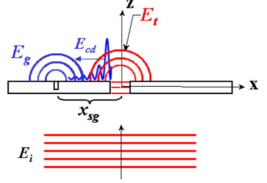
Figure 4. The incoming plane wave E_i propagates through the slit and launches surface waves along \pm x on the output-side surface. The composite wave E_{cd} , evanescent in z and indicated in blue, travel away from the slit until it encounters a groove where it is reconverted to propagating modes E_g that interferes with the propagating mode directly transmitted through the slit E_t . The interference pattern is detected in the far-field by a photodetector in the z \geq 0 half-space.
