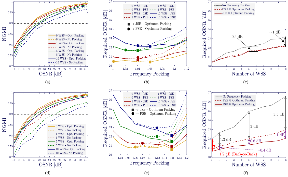
Fig. 4: Experimental results of effects of cascaded 75 GHz WSS filtering with frequency packing. (a)–(c) 0.12 roll-off, (d)–(f) 0.2 roll-off.
