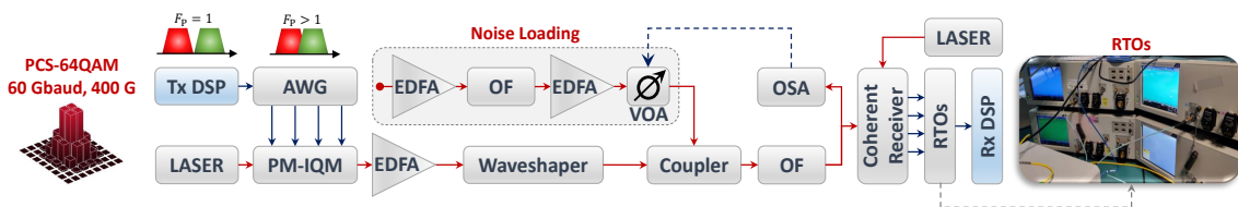
Fig. 3: Experimental setup with worst-case noise loading to evaluate the filtering penalties caused by cascaded WSS. OF: Optical Filter
