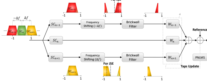
Fig. 2: JSE architecture. PNLMS: Power Normalized LMS
