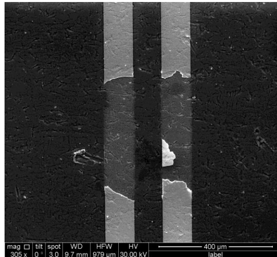
Figure 2.36: A 305x magnification SEM image of the insulated gold tracks of a stainless steel probe.
